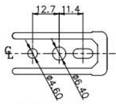
Detail T2 (2:1) ▲
