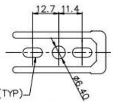
Detail T1 (2:1) ▲
