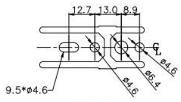
Detail U (2:1) ▲
